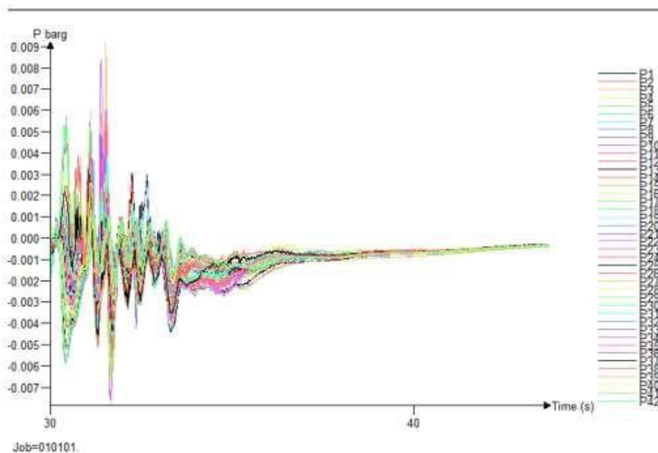
Figure 4: Pressure changes over time in FLACS simulation
